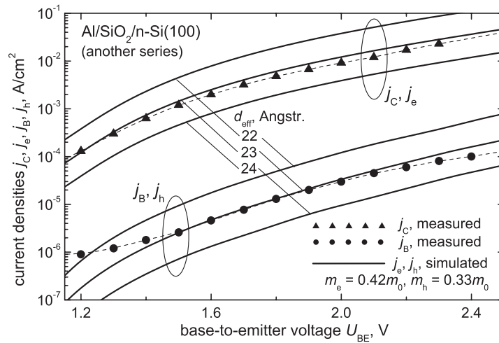
Figure 6. Estimation of the insulator thickness in a MOS tunnel emitter transistor from a series other than that used for figures 2–5. The coincidence of d_{\text{eff}} values obtained on the basis of the j_C and j_B curves speaks for an adequacy of the determined parameter m_h and of the model in general.
