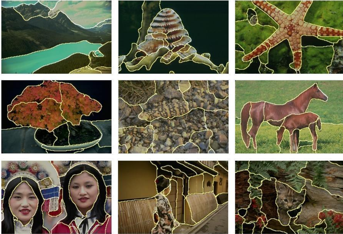
Image Segmentation
